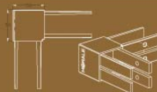
corner-connector: 133*133*50mm
